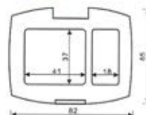
ES-195C SIZE:W82*65*H17mm
