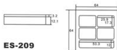
SIZE: W64*64*H15.3mm
