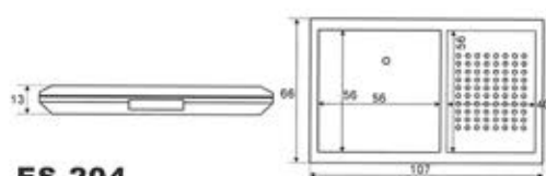
SIZE:W107*66*H13mm
