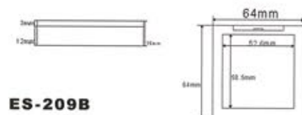
SIZE: W64*64*H15.3mm
