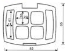
ES-195C SIZE:W82*65*H17mm
